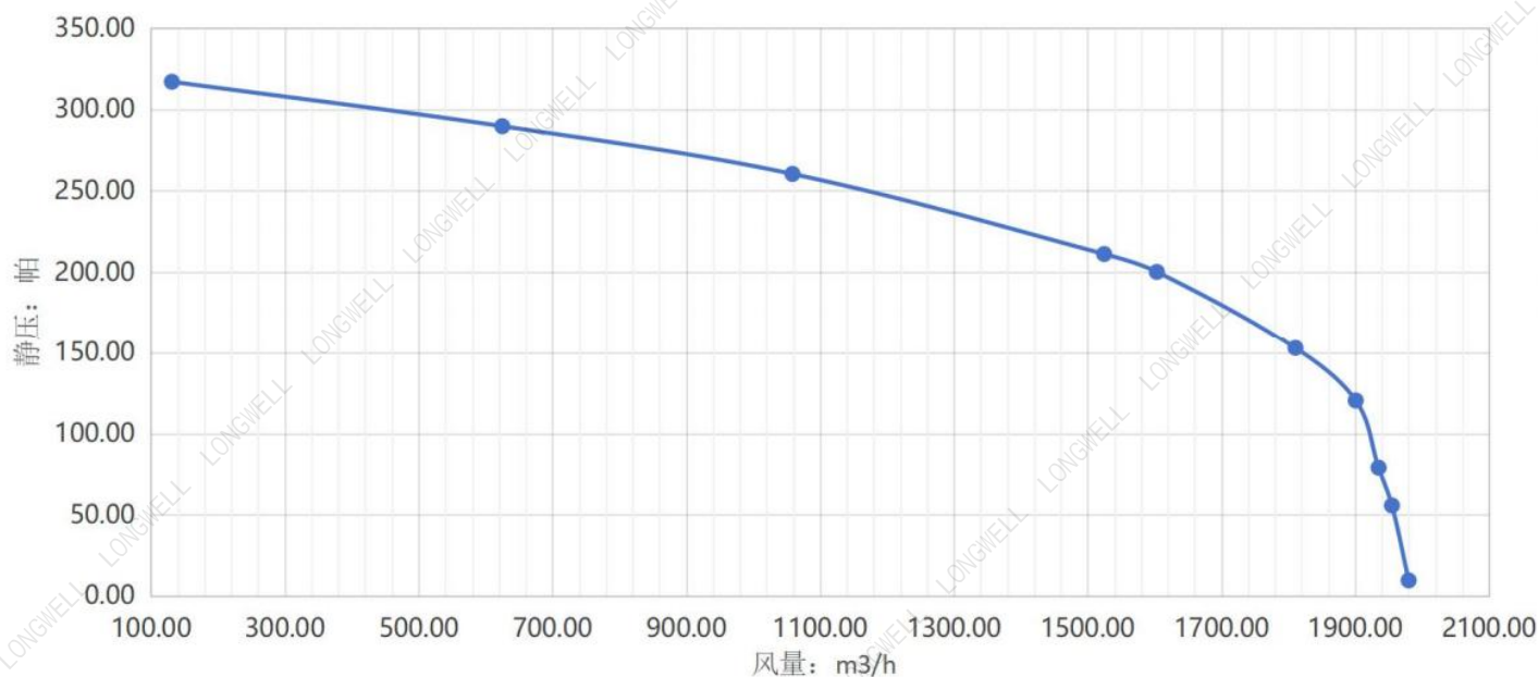
Charts :Air Flow (P-Q)
