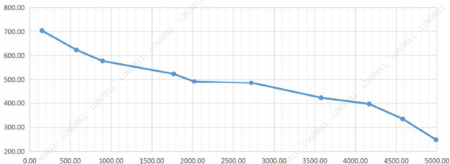
Charts :Air Flow (P-Q)
