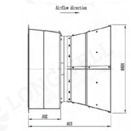
36"×50"with three blades
